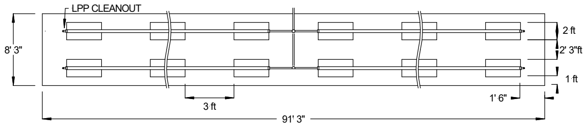
FIGURE 8: PLAN VIEW – EXAMPLE 2 - BED
