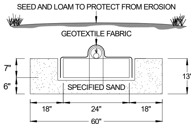
FIGURE 6: SECTION VIEW – EXAMPLE 1
