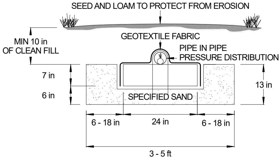
FIGURE 2: TYPICAL A42 CROSS SECTION
