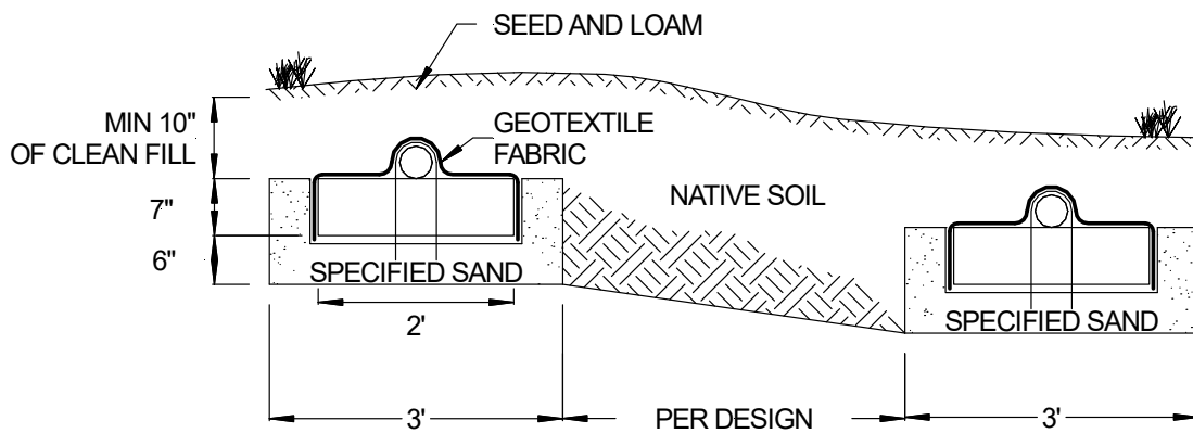
FIGURE 11: SECTION VIEW – TRENCH SYSTEM – SLOPING SITE
