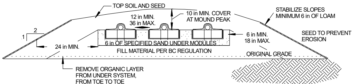
FIGURE 15: RAISED BED ON SLOPE
