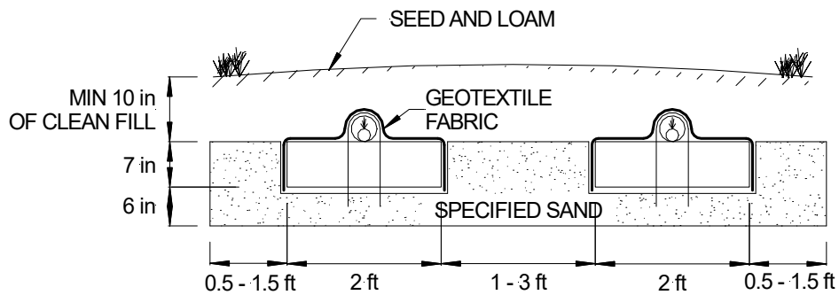
FIGURE 12: SECTION VIEW – BED SYSTEM EXAMPLE
