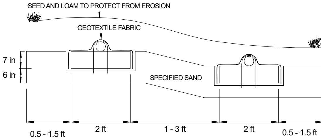
FIGURE 13: SECTION VIEW – 2 LATERAL BED SYSTEM; SLOPING SITE
