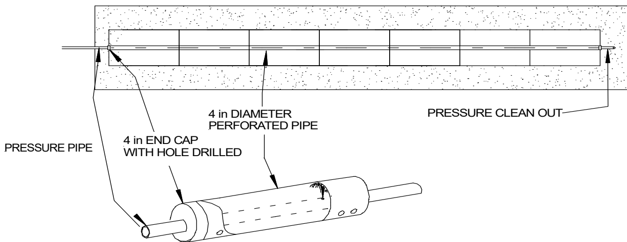
FIGURE 16: PRESSURE PIPE PLACEMENT
