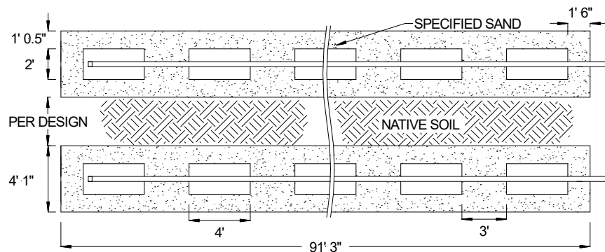
FIGURE 7: PLAN VIEW – EXAMPLE 2 – OPTION 1 TRENCHES
