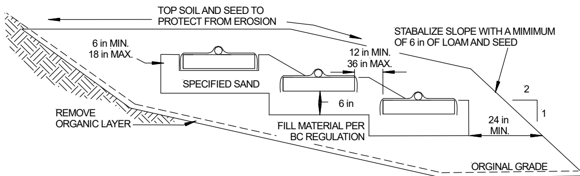
FIGURE 15: RAISED BED ON SLOPE
